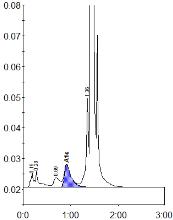
Peak table - ID: 10470097
